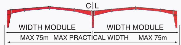
RSSLLP Multi Gable
