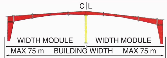
RSSLLP Multi Span-1
